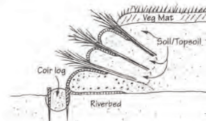
b) Brush Layering
