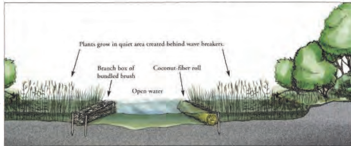
③ Alternatives using coir logs for securing toe of slope depending upon site:
